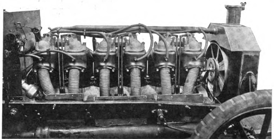
SIX-CYLINDER 80-HORSEPOWER MOTOR MOUNTED IN NAPIER RACING CAR.
